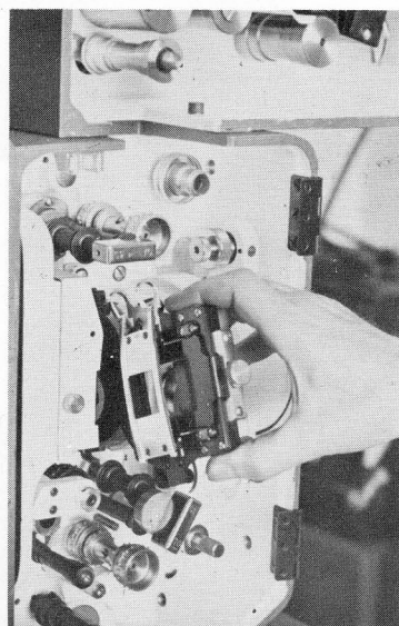
REMOVE 70 MM FILM GATE
