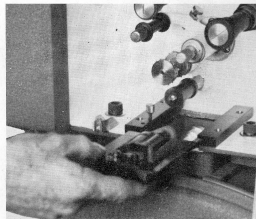
INSTALL THE 35 MM UPPER & LOWER FIRE TRAP ROLLER HOLDERS AND . . .
