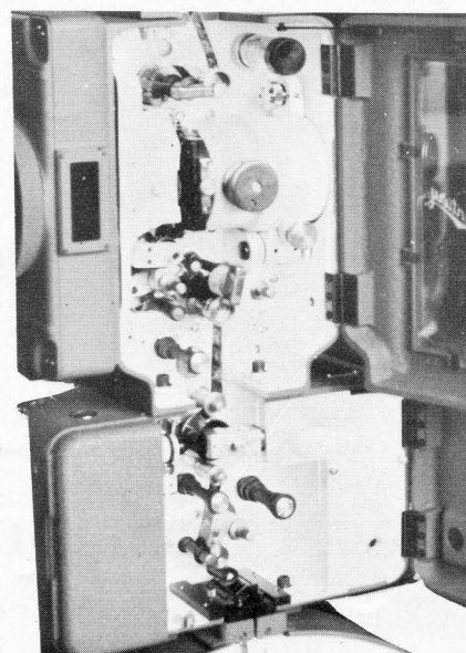
PASSING THROUGH THE OPTICAL REPRODUCER..
