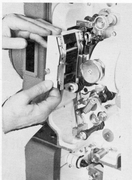
REMOVE 70 MM FILM TRAP
