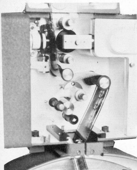
BY-PASSING THE OPTICAL REPRODUCER
