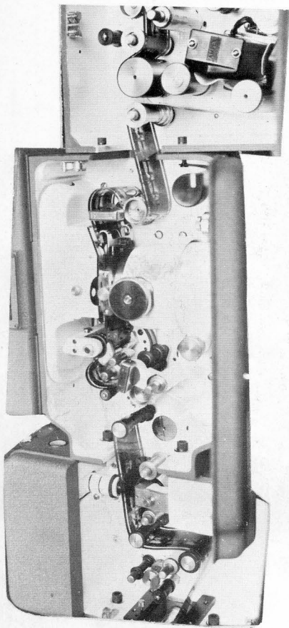
THREADING THE PROJECTOR FOR 70 MM FILMS
