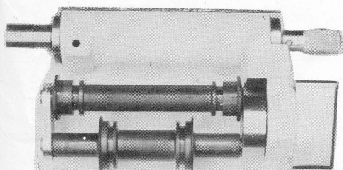
REMOVE 70 MM FILM TRAP
