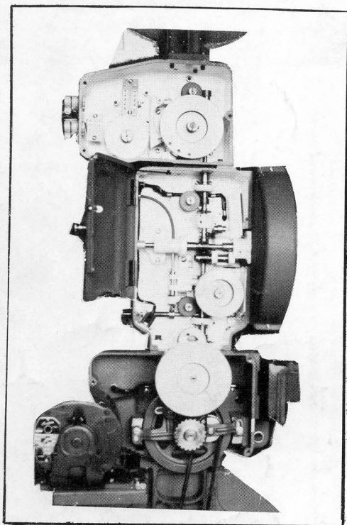
THE CENTURY 70/35 MM PROJECTOR (DRIVE SIDE)
