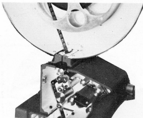
BY-PASSING THE MAGNETIC REPRODUCER
