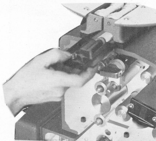
INSTALL THE 35 MM UPPER & LOWER FIRE TRAP ROLLER HOLDERS AND . . .
