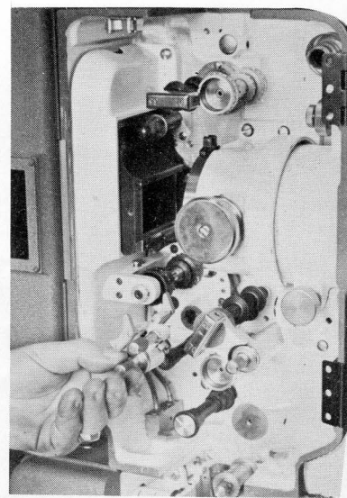
REMOVE 70 MM INTERMITTENT SPROCKET PAD ASSEMBLY . . .
