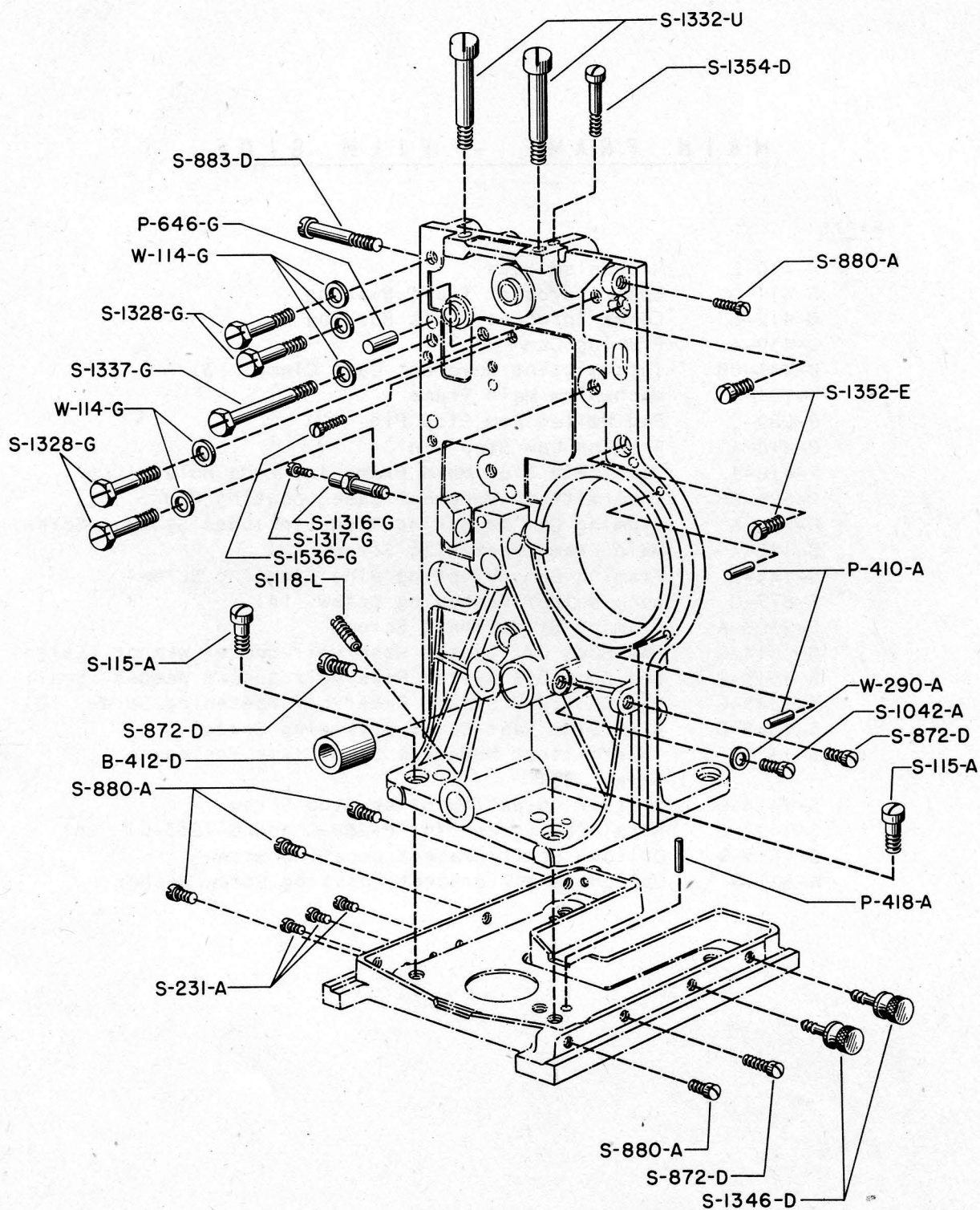
MAIN FRAME — GEAR SIDE
